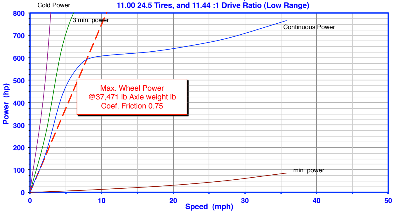
RS-110K Drawbar Pull 11.00 24.5 Tires, and 11.44:1 Drive Ratio (Low Range)
