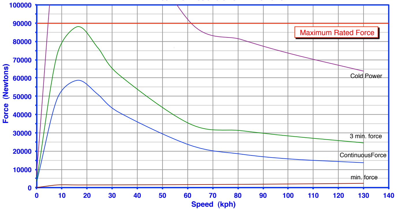
RS-80K Drawbar Force 11.00 24.5 Tires and 5.13:1 Drive Ratio
