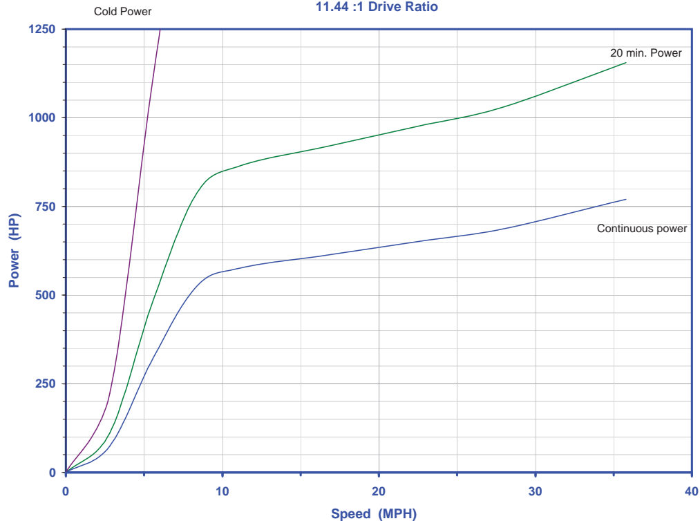
RS-80K Power Absorption 11.44 :1 Drive Ratio
