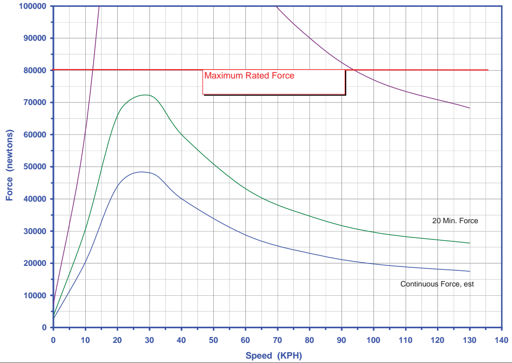
RS-80K Drawbar Force 5.13:1 Drive Ratio
