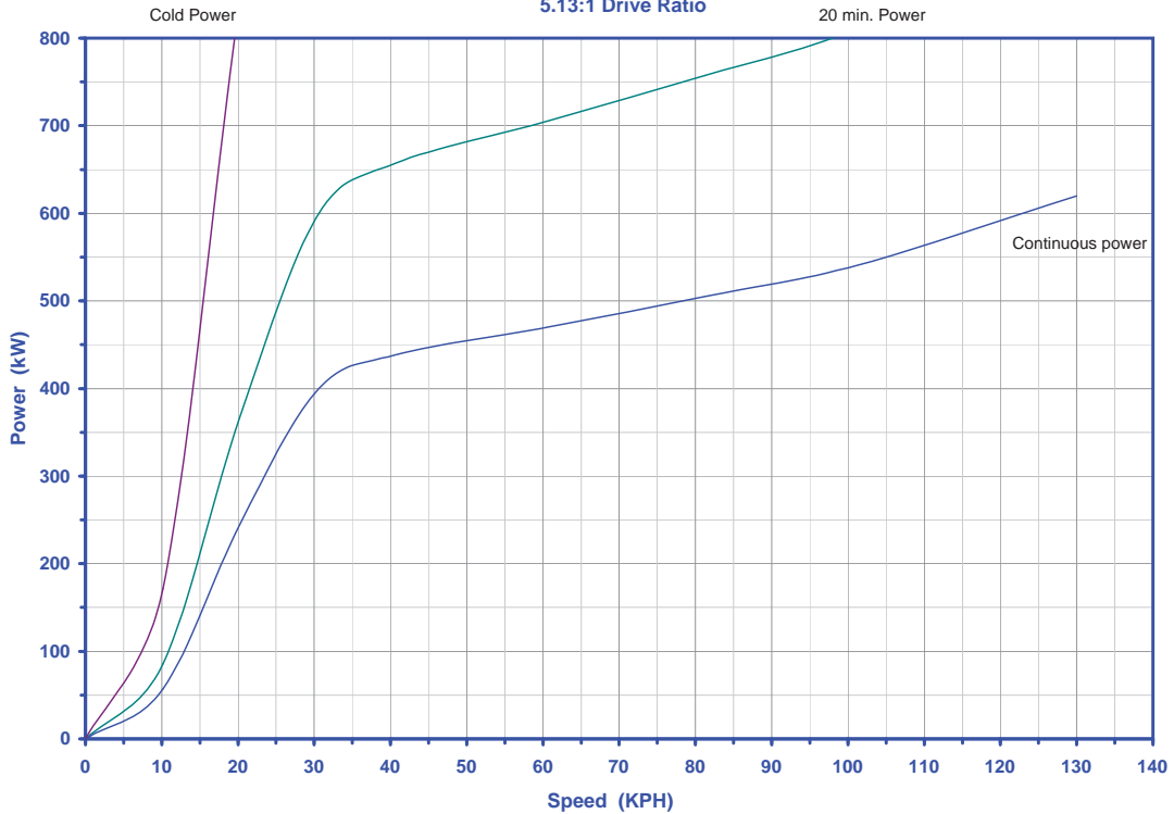
RS-80K Power Absorption 5.13:1 Drive Ratio
