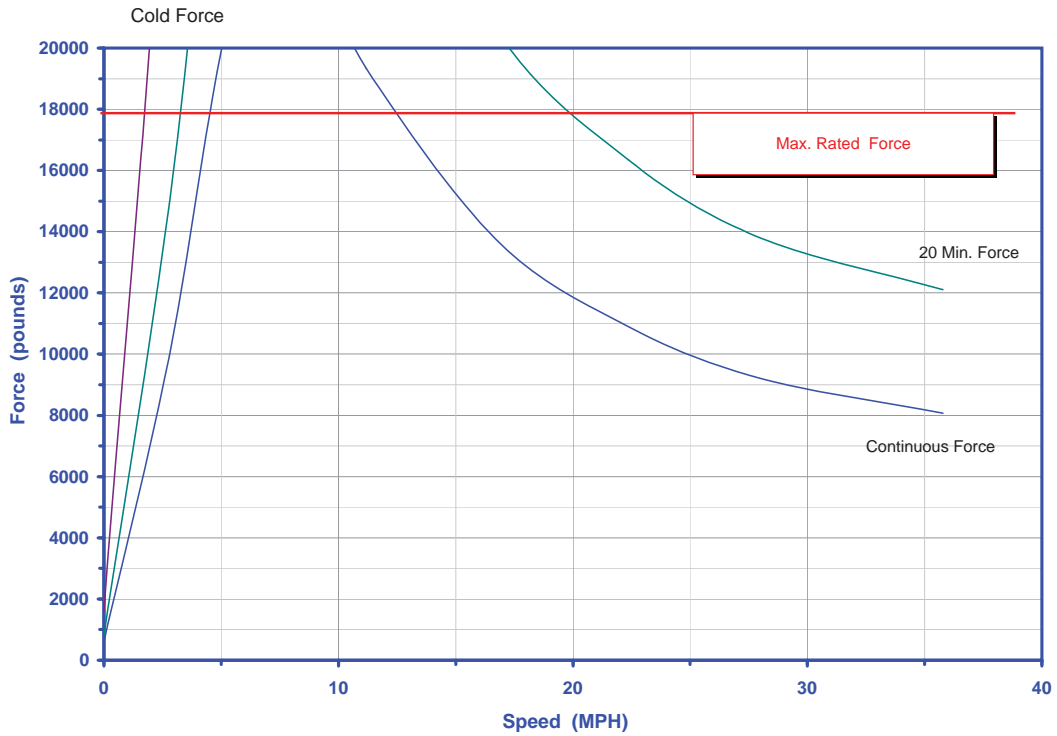
RS-80K drawbar pull 11.44:1 Drive Ratio
